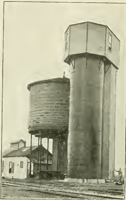
KENNICOTT WATER SOFTENING PLANT.
